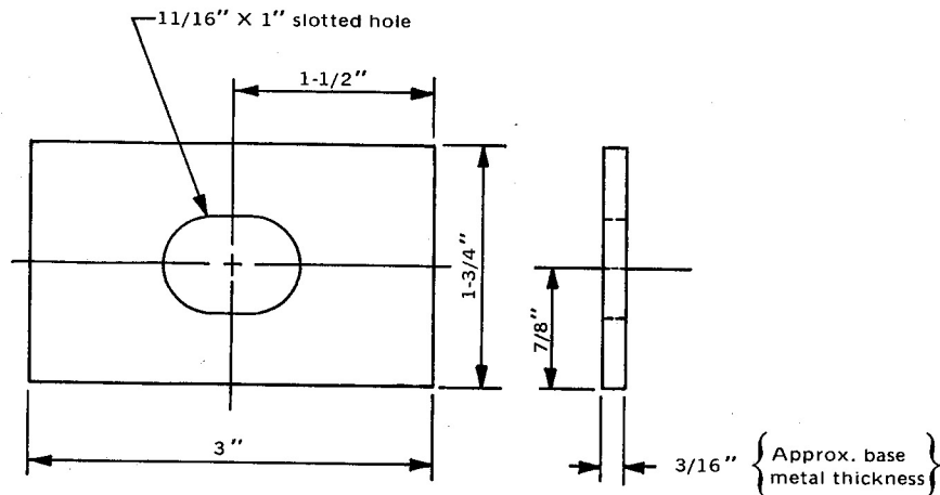
WASHER
